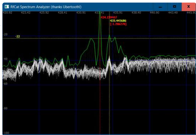
Figure 1. Affichage du spectre Rfcat.
