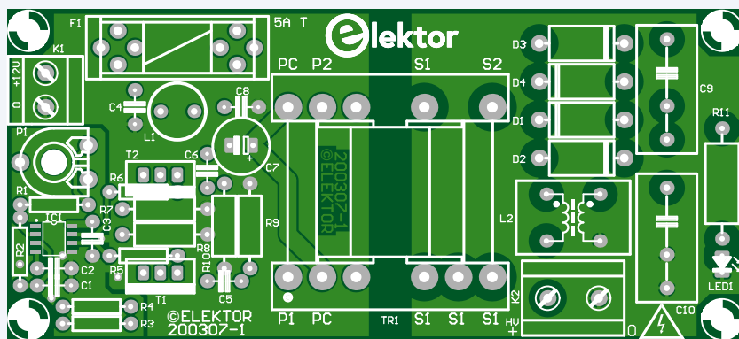
Figure 4. Circuit imprimé.
